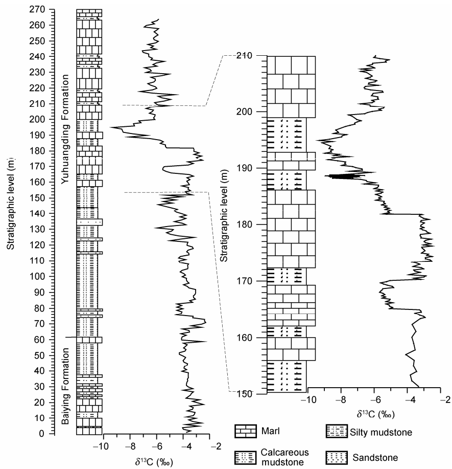
Figure 2 Lithostratigraphic column and carbon isotope record of the Yuhuangding section.
