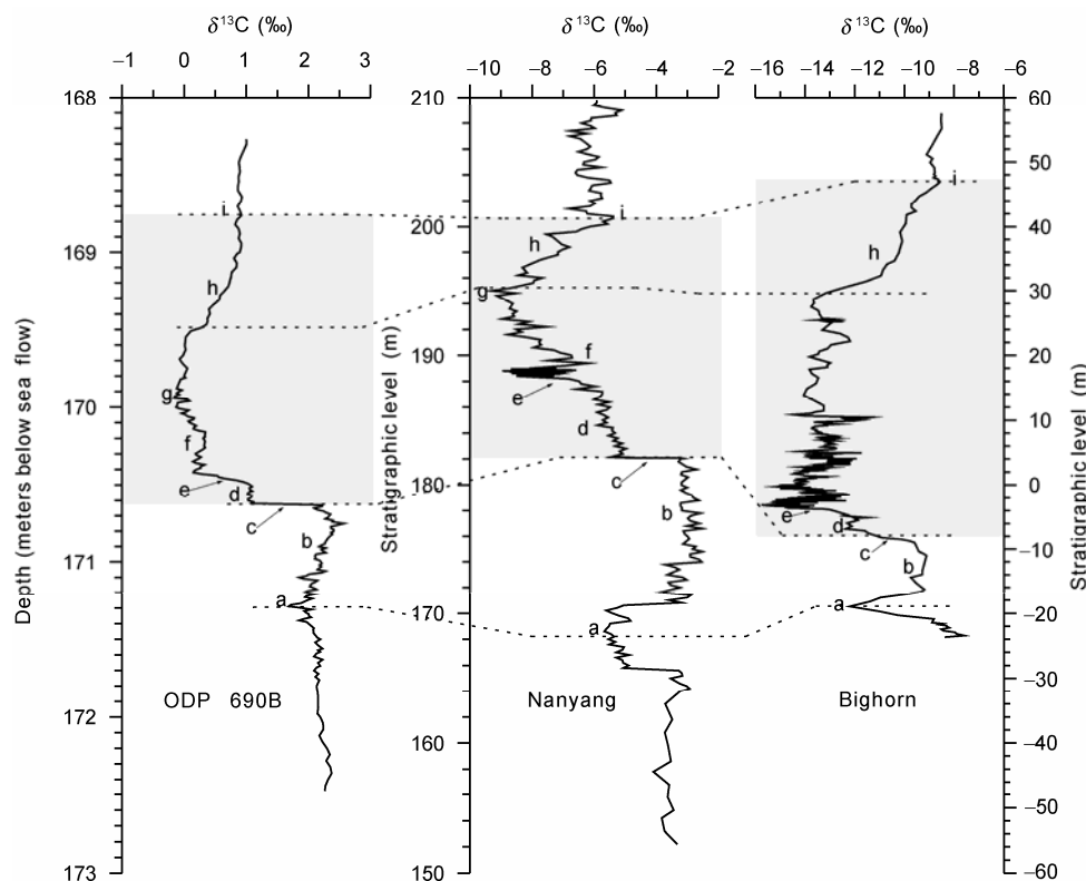
Figure 3 Correlation of \delta^{13}\text{C} records between ODP 690B [10], Nanyang Basin, and Bighorn Basin [19]. ODP 690B data are from bulk carbonates, and are plotted against depth as meters below the seafloor. Bighorn Basin data are derived from pedogenic carbonate nodules. Shaded areas indicate the PETM event.
