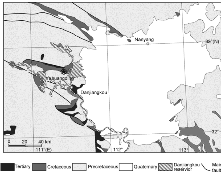
Figure 1 Geological sketch map of the Nanyang Basin.
